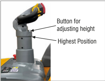
Tiller height can be adjusted by 6 level,lowest height 1040mm
